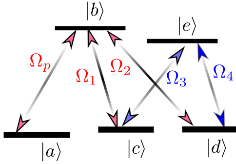
Figure 1. Schematic diagram of the five-level Lambda-tripod quantum system.
