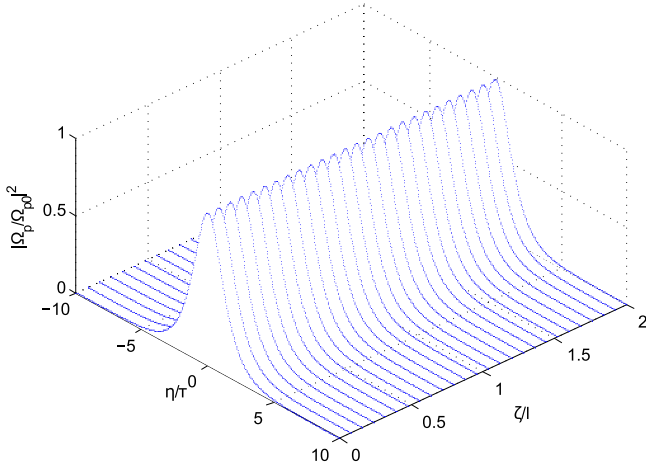
Figure 6. Propagation dynamics of an ultraslow optical soliton with \tau = 10^{-7} s, l = 1 cm, and \eta = 1.0 \times 10^{10} cm ^{-1} s ^{-1} and the parameters given in the main text.
